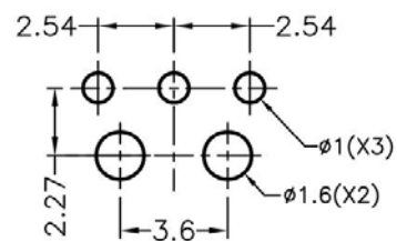
MOUNTING HOLES
